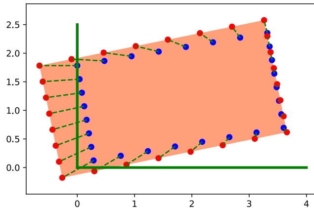
Figure 4.17 - The convex approximation to the constrained pose estimation problem with known correspondences. I have added constraints that both the x and y positions of all of the points in the estimated pose must be greater than 0 in the world frame (as illustrated by the green lines).
