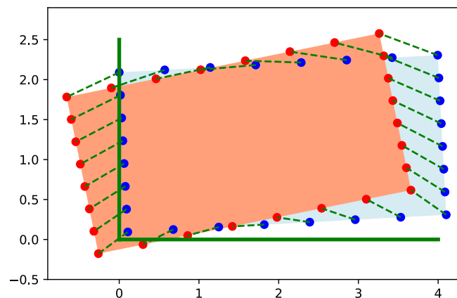
Figure 4.16 - The solution to the constrained pose estimation problem with known correspondences. I have added constraints that both the x and y positions of all of the points in the estimated pose must be greater than 0 in the world frame (as illustrated by the green lines). The red scene points are in penetration, but the solver returns the pose illustrated by the blue, which satisfies the constraints.
