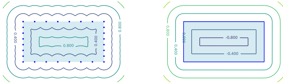
Figure 4.14 - Contour plot of the distance function for our point-based representation of the rectangle (left), and the signed distance function for our "mesh-based" 2D rectangle. The smoother distance contours in the mesh-based representation can help alleviate some of the local minima problems we observed above.
