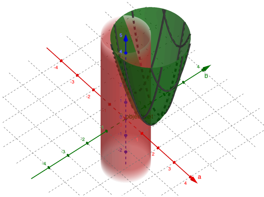
Figure 4.4 - The x and y axes of this plot correspond to the parameters a , and b , respectively, that define the 2D rotation matrix, R . The green quadratic bowl is the objective \sum_i \|R \mathcal{O} p^{m_{\mathcal{C}_i}} - p^{s_i}\|^2 , and the red open cylinder is the rotation matrix constraint. Click here for the interactive version.
