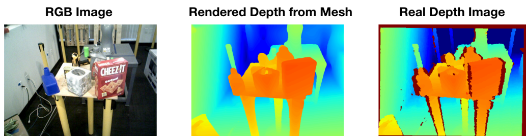
Figure 4.2 - Real depth sensors are messy. The red pixels in the far right image are missed returns -- the depth sensor returned "maximum depth". Missed returns, especially on the edges of objects (or on reflective objects) are a common sighting in raw depth data. This figure is reproduced from [2].
