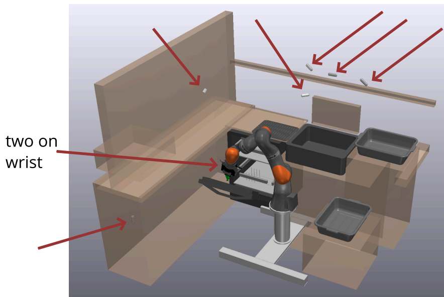
Figure 4.3 - When luxury permits, we try to put as many cameras as we can into the robot's environment. In this dish-loading testbed at TRI where we put a total of eight cameras into the scene (it still doesn't resolve the occlusion problem).
