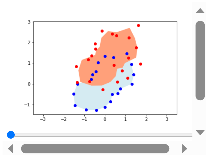
Figure 4.8 - A sample run of ICP with Gaussian noise added to the positions of the scene points.
