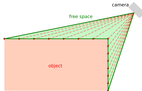
Figure 4.18 - The rays cast from the camera to the depth returns define a "free space obstacle" that other objects should not penetrate.
