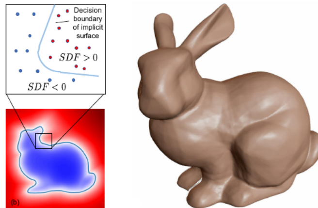
Figure 4.15 - A visualization of a "signed distance function" (SDF) representation of 3D geometry. Reproduced with permissions from [3].
